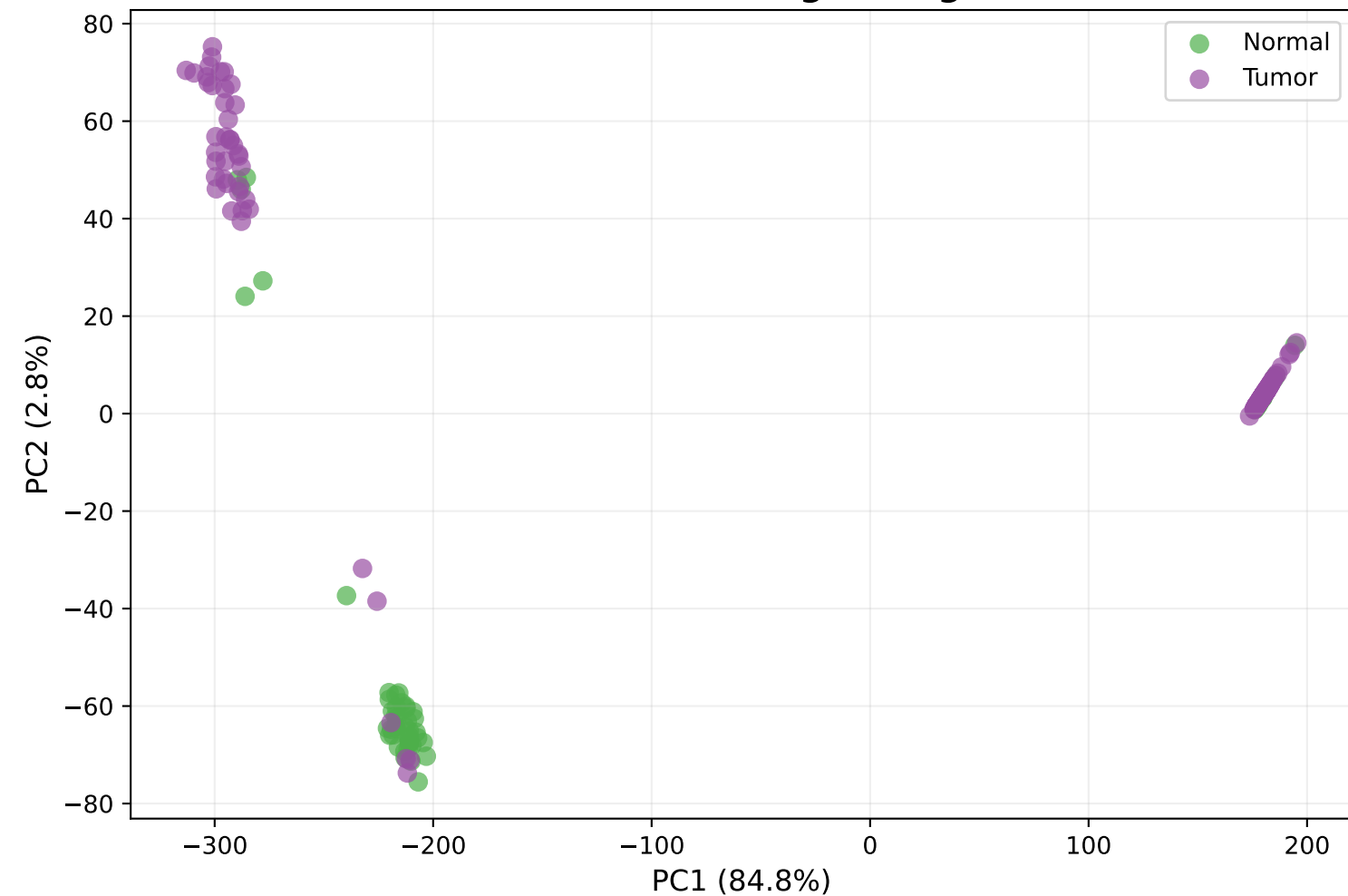
B: After Normalization (Biological Signal Dominant)
