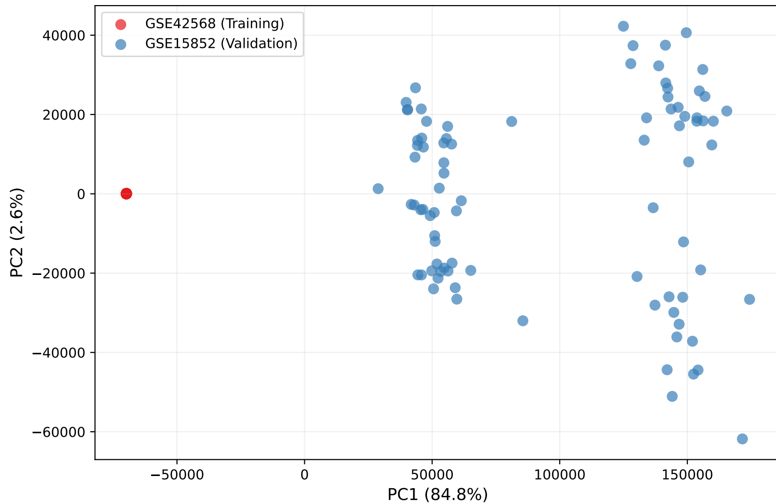
A: Before Normalization (Batch Effect Visible)
